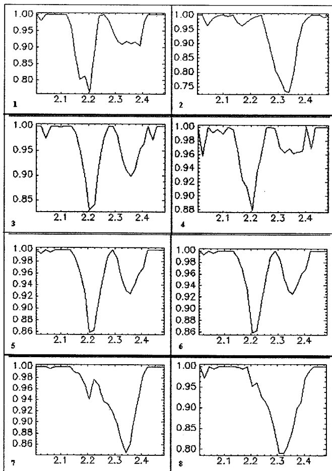
Figure 6. MTFM input end-members. These included the following (1) Kaolinite (2) Calcite, (3) Illite, (4) Kaosmectite, (5) Montmorillonite, (6) Muscovite, (7) Epidote, and (8) Chlorite.
