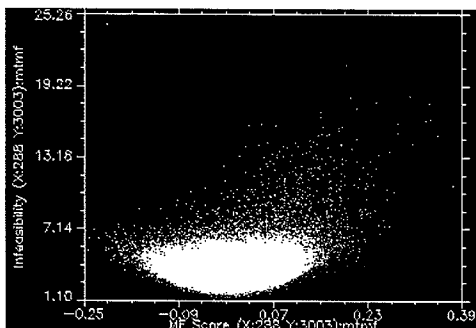
Figure 7. Scatter plot of an MF band and Infeasibility band. The gray area in the lower-right area represents pixel values with a high probability of being an end-member mineral.
