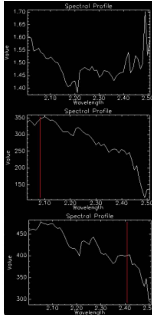
Figure 4. Kaolinite and unknown mineral mixed spectrum.
