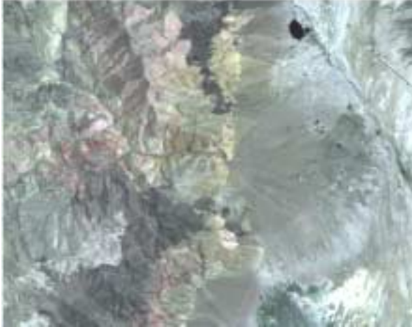
Figure 1. AVIRIS RGB image of the Dixie Valley study area.
