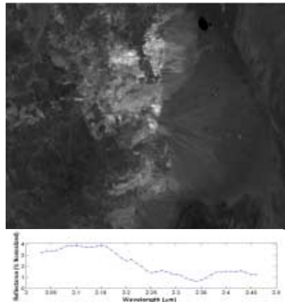
Figure 8. PVA End-Member 2 gray-scale abundance map, and spectra. Black pixels on map indicate absence of this spectrum. White pixels indicate maximum observed in the image (59%).
